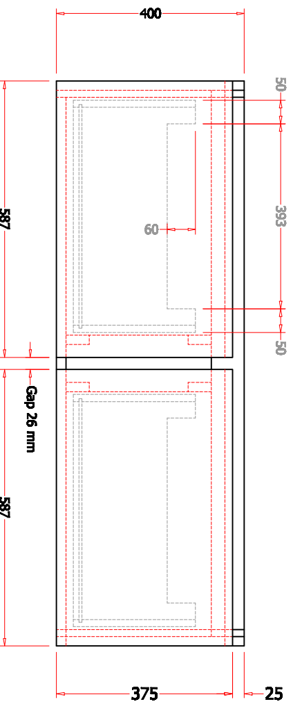
FRONT VIEW
